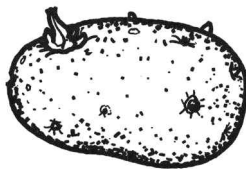
MARINER 9 IMAGE OF PHOBOS
