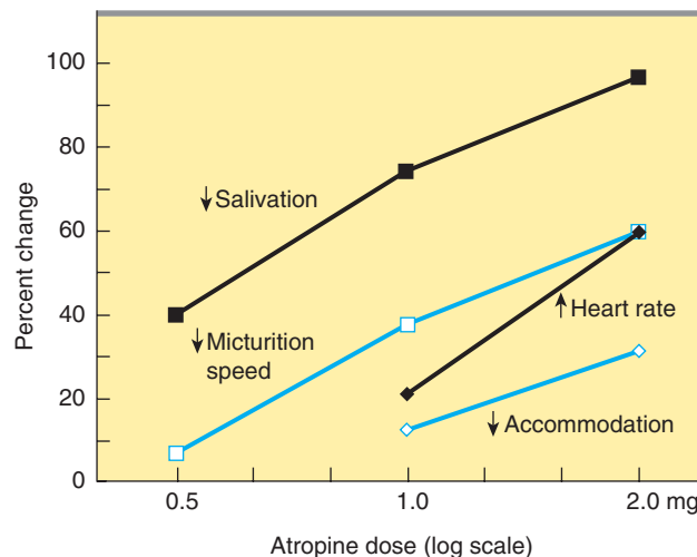
FIGURE 8–6 Effects of subcutaneous injection of atropine on salivation, speed of micturition (voiding), heart rate, and accommodation in normal adults. Note that salivation is the most sensitive of these variables, accommodation the least. (Data from Herxheimer A: Br J Pharmacol 1958;13:184.)
